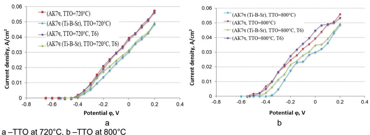
Figure 8 – Polarization curves of AK7ch and AK7ch(Ti-Sr-B) alloys in the additionally heat-treated state after testing in an aqueous solution of 3% NaCl + 1% HCl
