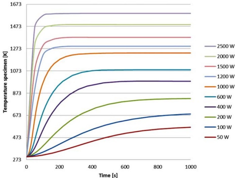
Fig. 4. Calculated temperatures of the specimen vs. time and input power.
