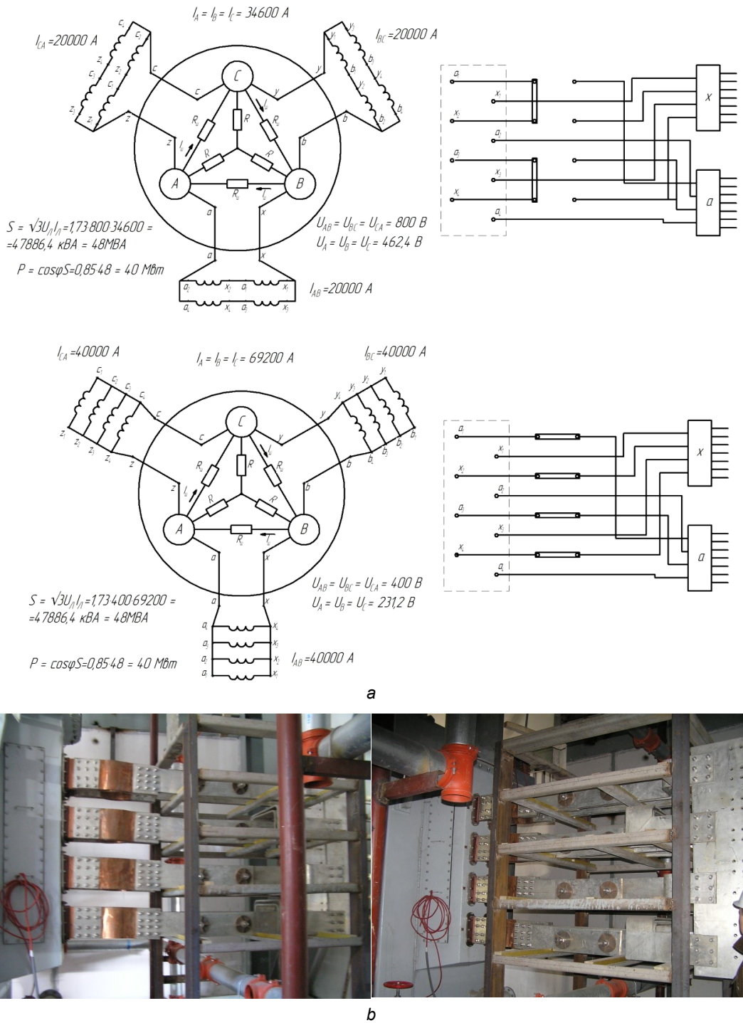
Fig. 9. Short network switching: a – diagram; b – general view.
