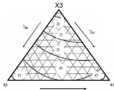
Fig. 2. Mathematical model of the of the impregnating pitch softening temperature dependence on the FF mass fraction.
